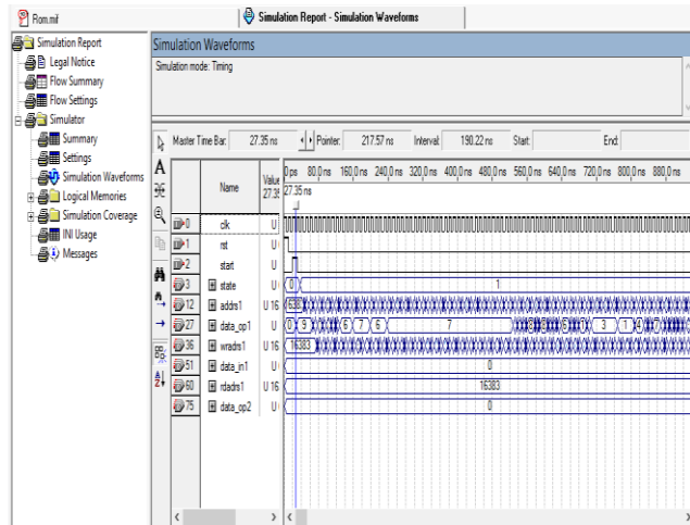
Figure 8. Simulation waveforms
