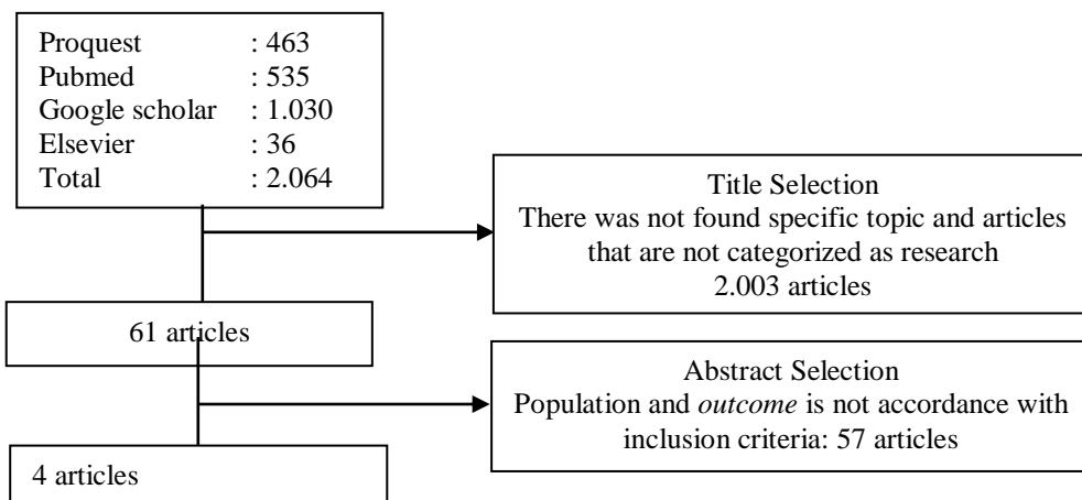
Figure 2. Search flow
