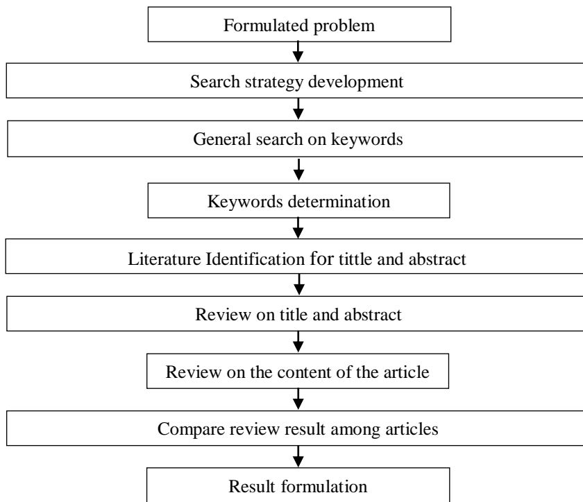
Figure 1. Research flow
