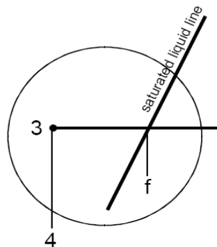
Figure 17. Condenser sub-cooling
