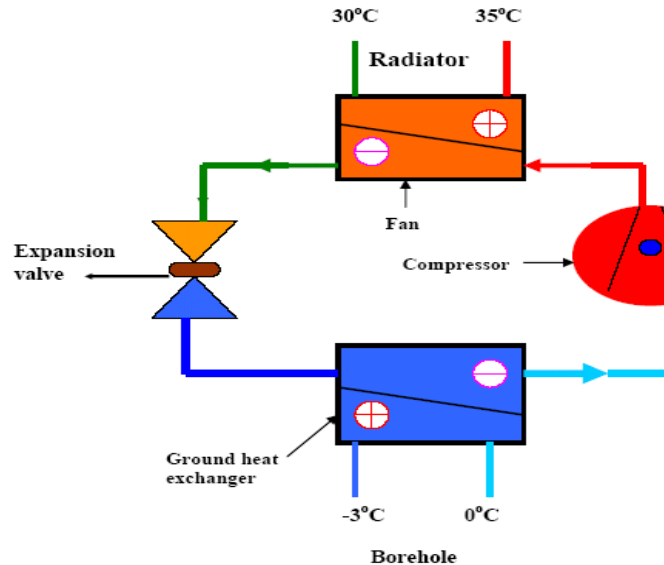
Figure 2. Detail of the GSHP circuit
