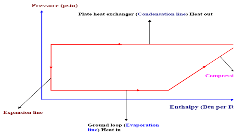
Figure 12. The ideal cycle on Pressure-Enthalpy diagram
