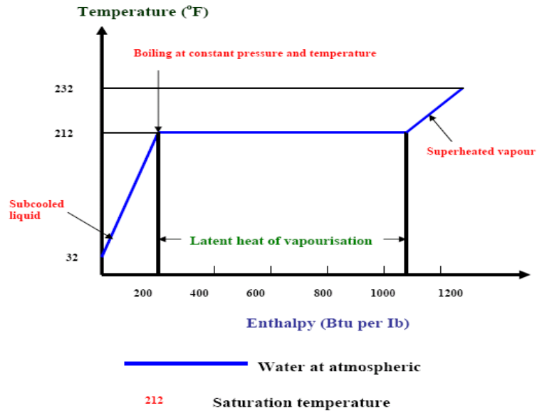
Figure 13. Water undergoing a change of the state
