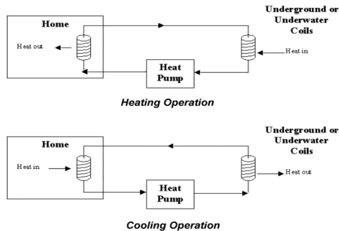
Figure 10. Heating and cooling operations
