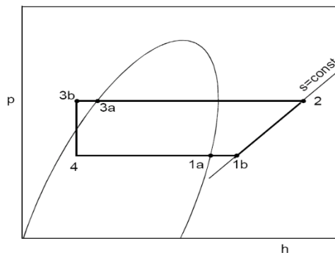
Figure 19. Diagram of liquid-suction heat exchanger
