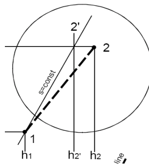
Figure 16. Isentropic compressor.
