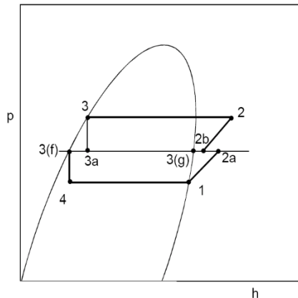
Figure 21. The cycle of multiple compressions using the flash chamber
