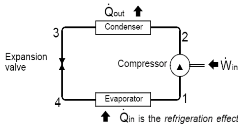
Figure 7. Simplified refrigeration system diagram
