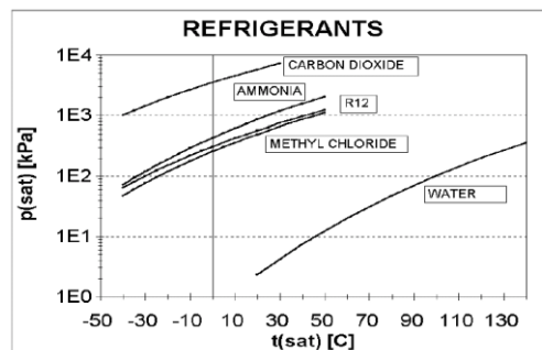
Figure 9. Refrigerant chart
