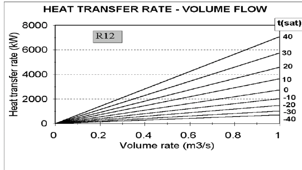
Figure 5. Heat transfer rate versus volume rate
