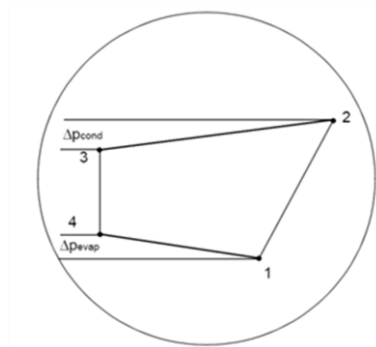
Figure 18. Pressure drops in evaporator and condenser
