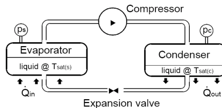
Figure 8. Heat pump refrigeration cycle
