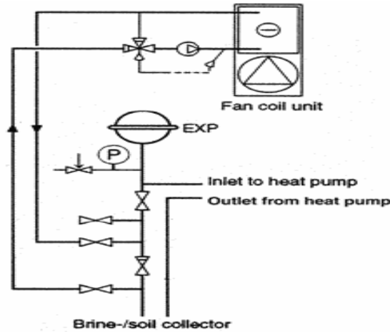
Figure 3. Diagram of the cooling system.
