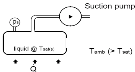
Figure 4. Refrigeration Cycle
