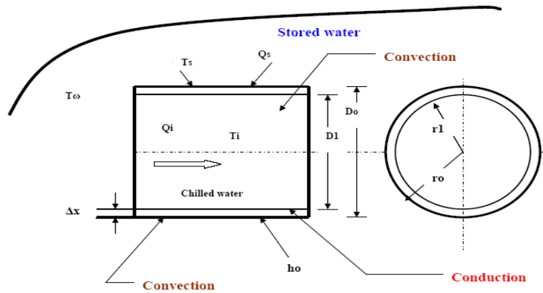
Figure 11. Schematic of heat transfer through a circular tube heat exchanger
