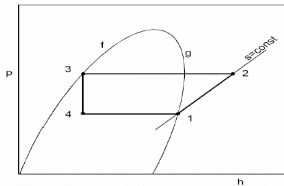
Figure 14. Refrigeration cycle
