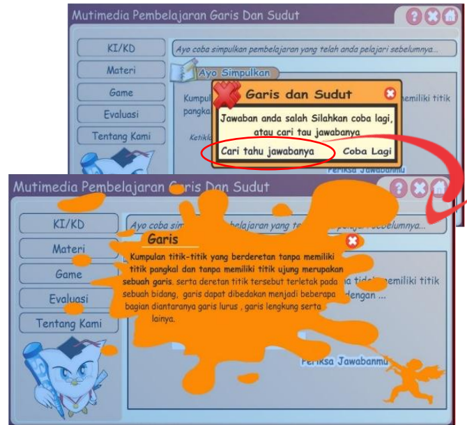
Figure 7. Conclusion page
