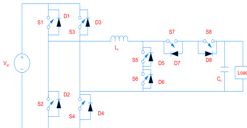
Figure19. Quazi ZSource Inverter
