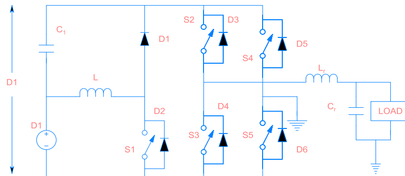
Figure 14. High step-up dc-to-dc converter
