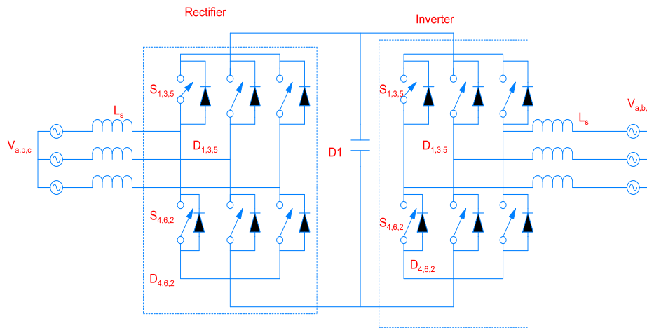
Figure 20. Bidirectional symmetrical DC–DC resonant converter
