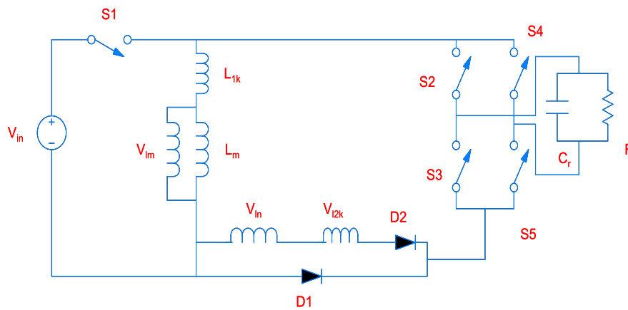
Figure 21. Single-stage conversion structures of Converters
