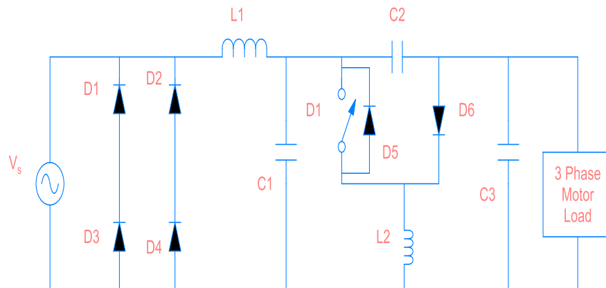
Figure15. Active buck–boost inverter
