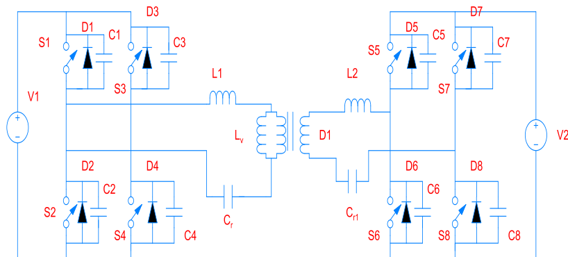
Figure17. Two-level, three-phase, back-to-back converter
