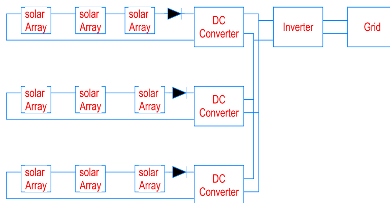
Figure 2. Multistring PCS
