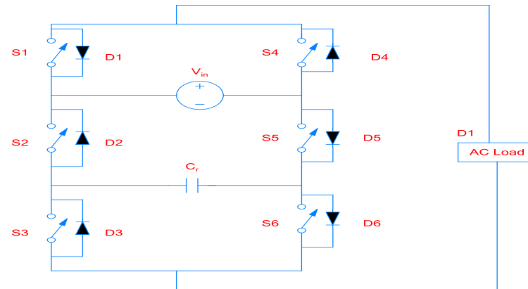
Figure18. Landsman converter
