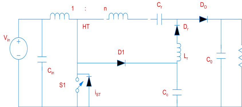
Figure7. Hybrid transformer dc-dc converter
