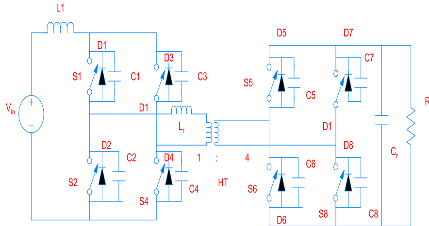
Figure 11. Dual-output DC-DC asymmetric buck converter
