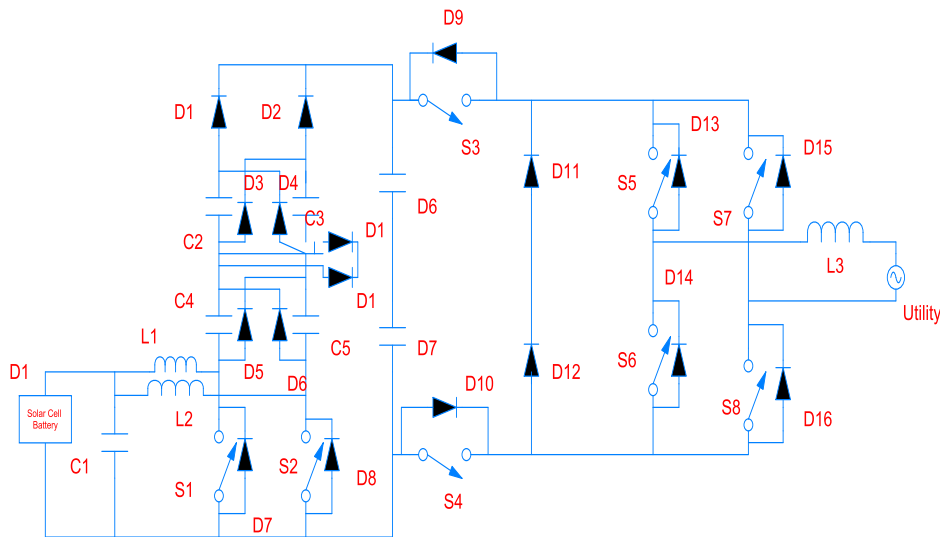
Figure10. two-step start up boost dc-dc converter
