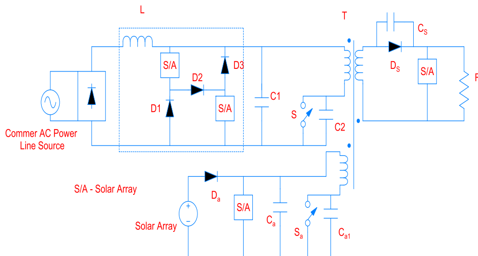
Figure 4. Buck–boost-type two-input dc–dc converter
