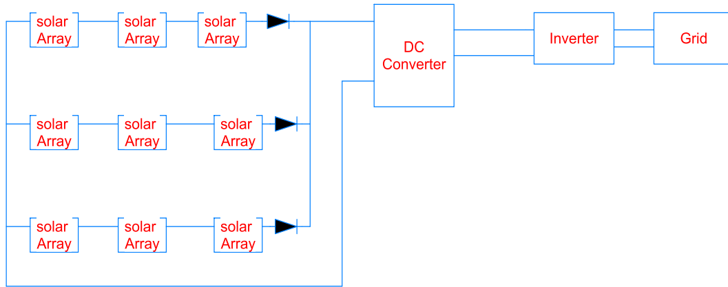
Figure 3. Centralized PCS
