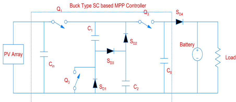
Figure 6. Switched capacitor dc-dc converter
