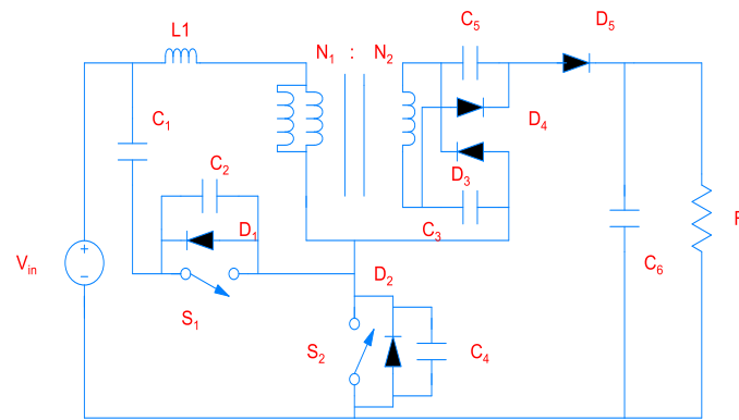
Figure13. Interleaved boost dc–dc converter
