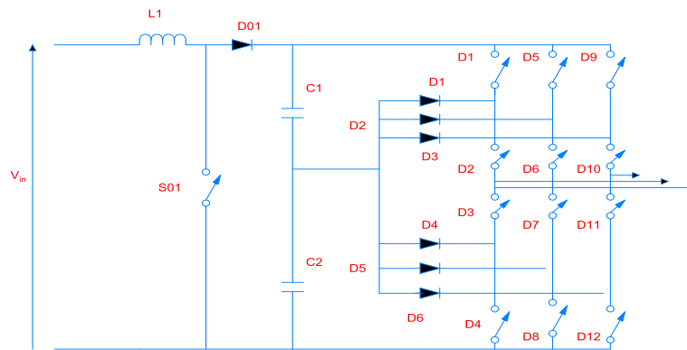
Figure16. Five-level packed U-cell inverter
