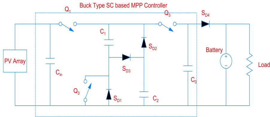
Figure 5. Fourth-order buck converter
