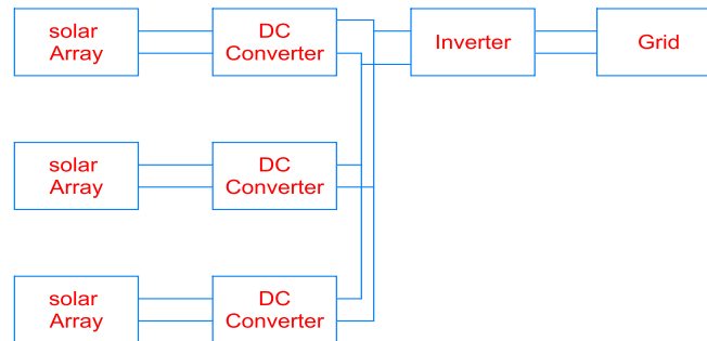
Figure 1. (MIC) with a central inverter
