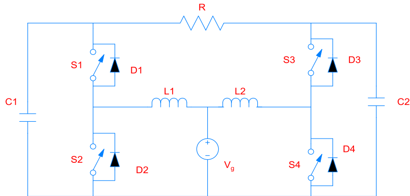
Figure 22. Grid-tied differential boost inverter
